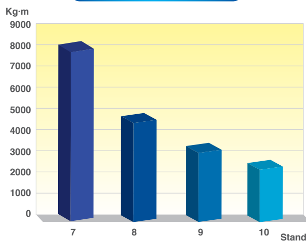
Rolling Torque
